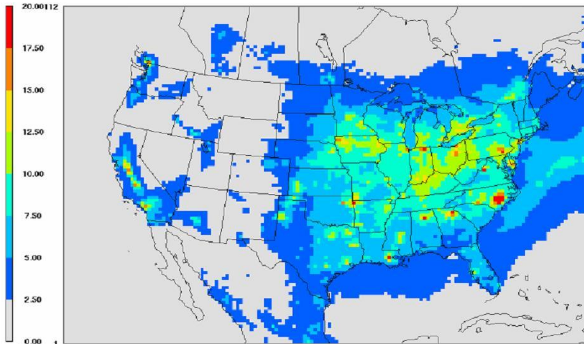
Figure 4-18. Estimated 2001 annual total deposition of nitrogen (kg-N/ha) to North America and adjacent coastal ocean.
