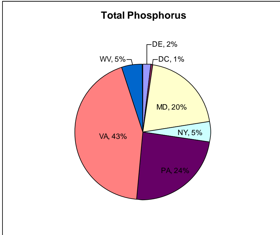
Figure 4-2. Model estimated total phosphorus loads delivered to the Chesapeake Bay by jurisdiction in 2009.
