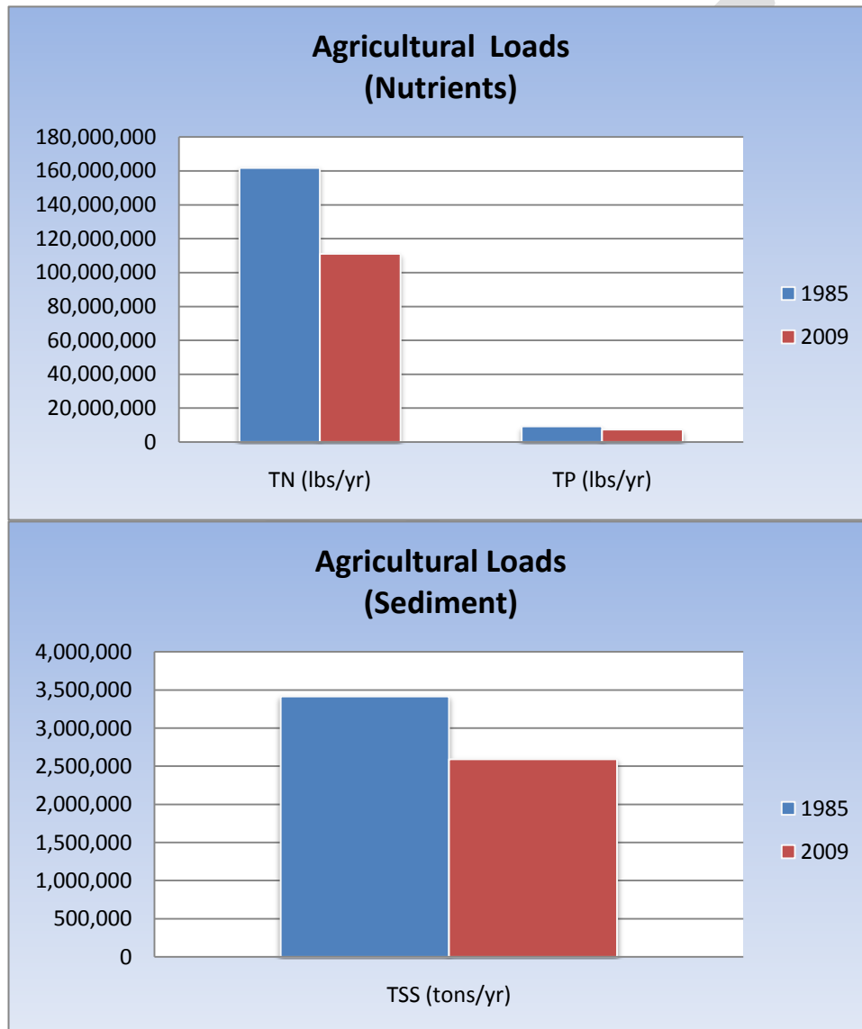
Figure 4-13. 1985 and 2009 modeled total nitrogen, phosphorus, and sediments loads from agricultural lands across the Chesapeake Bay watershed.
