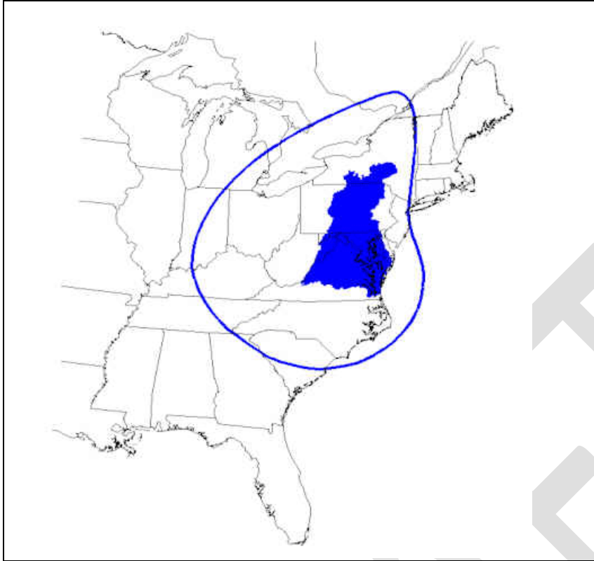
Figure 4-16. Principle area of NO x emissions (outlined in blue) that contribute nitrogen deposition to the Chesapeake Bay and its watershed (solid blue fill) (the Bay airshed).
