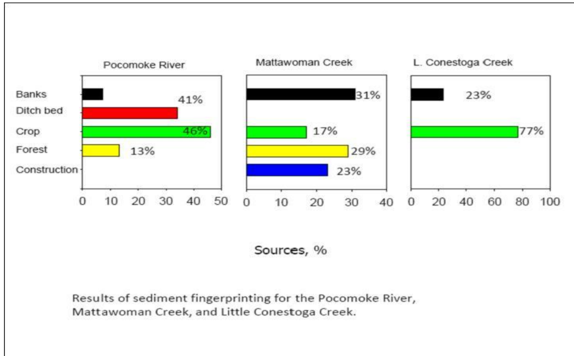
Figure 4-19. Relative estimates of sources of erosion from land sources (crop, forest, or construction) or bank sources banks and ditch beds).
