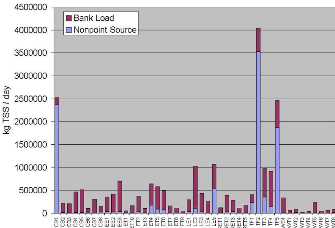
Figure 4-21. Estimated tidal sediment inputs for 1990 from the Chesapeake Bay watershed and from shore erosion. Shoreline sediment inputs (here labeled bank load) are estimated to be about equal to watershed inputs (here labeled as nonpoint source).
