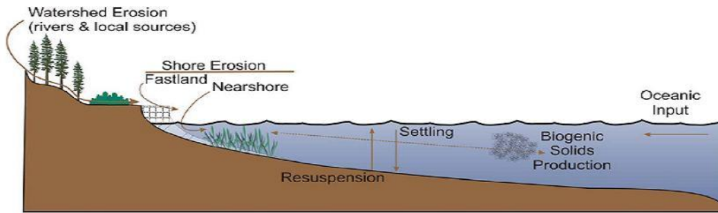
Figure 4-20. Sources of total suspended solids in the Chesapeake including the two components of shoreline erosions, fastland and nearshore erosion.
