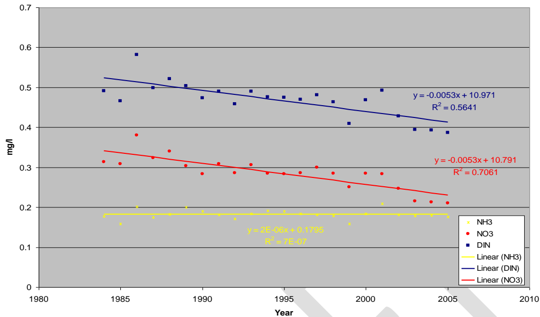
Figure 4-17 Trend of estimated average nitrate and ammonia deposition concentrations in the Phase 5 Model domain from 1984 to 2005. .
